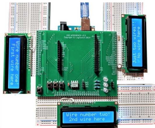
Example Wireless Breadboarding with the WorkBench
